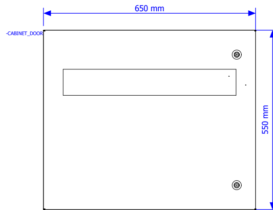
DOOR VIEW
