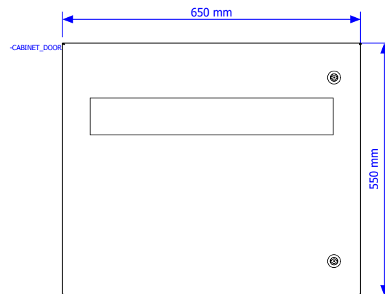
DOOR VIEW
