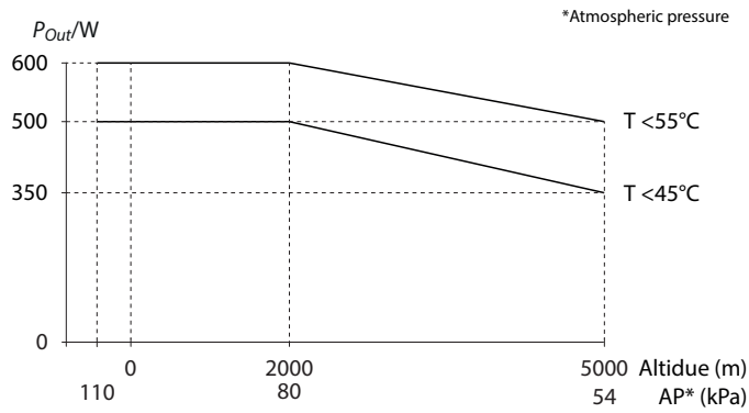
Fig. 19: Derating – output power vs. altitude
