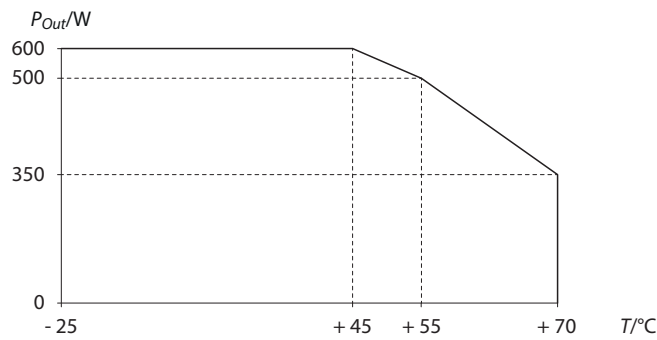
Fig. 22: Derating – standard mounting orientation
