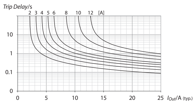
Fig. 17: Trip curve diagram (max. 12 A)
