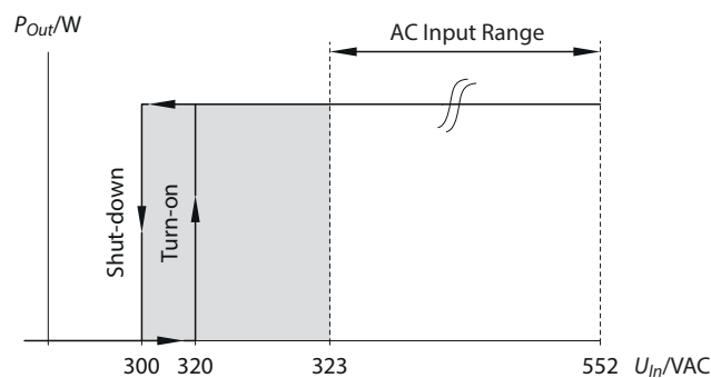
Fig. 13: Voltage range – input voltage AC
