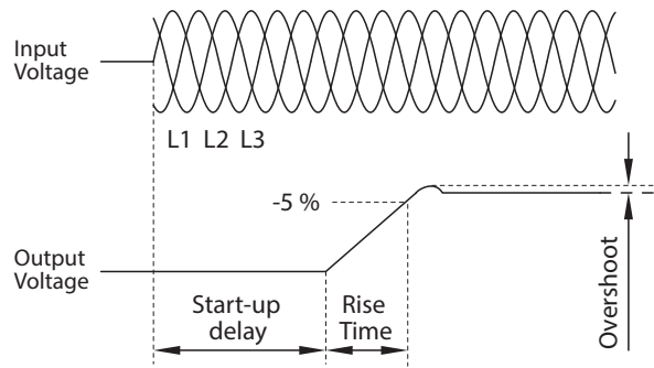
Fig. 14: Switch-on behavior
