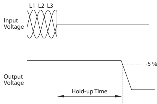
Fig. 9: Shutdown behavior
