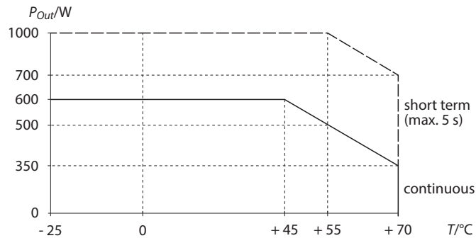
Fig. 18: Derating – output power vs. ambient temperature
