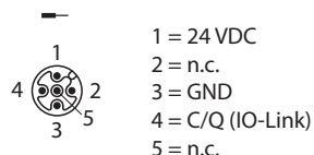
Fig. 12: Pin assignment - IO-Link interface (X0)
