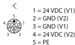
Fig. 11: Pin assignment — M12 connector, DC output voltage side (XD2, XD3)
