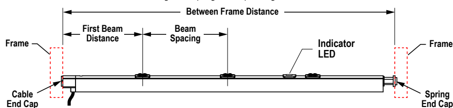
Figure 2. T-Slot Configuration
