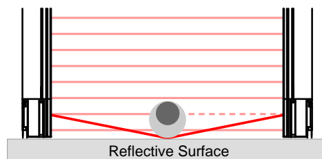
Figure 8. Determining Worst-Case Resolution With Larger Test Piece
