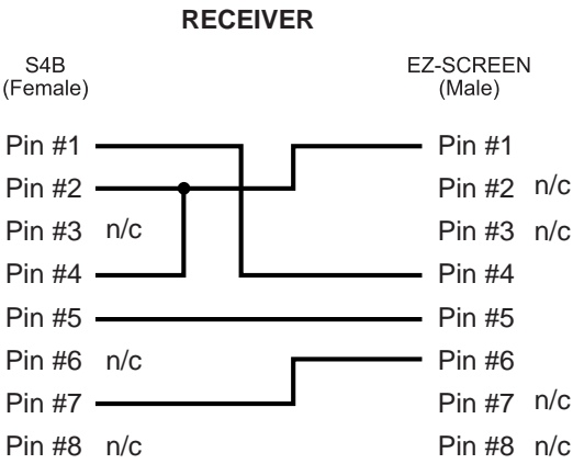
Figure 40. Receiver Wiring Diagram
