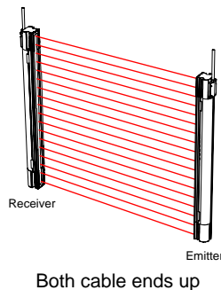
Figure 10. Examples of Correct Emitter/Receiver Orientation
