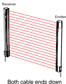
Figure 10. Examples of Correct Emitter/Receiver Orientation
