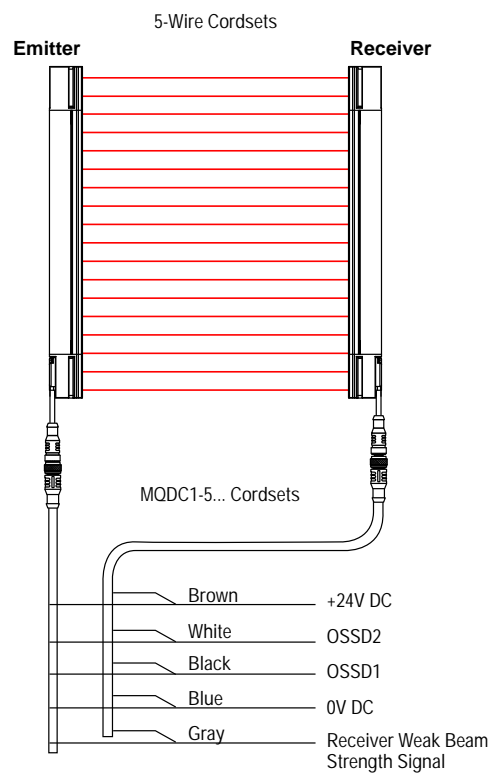
Figure 25. Individual Cordsets: 5-Wire
