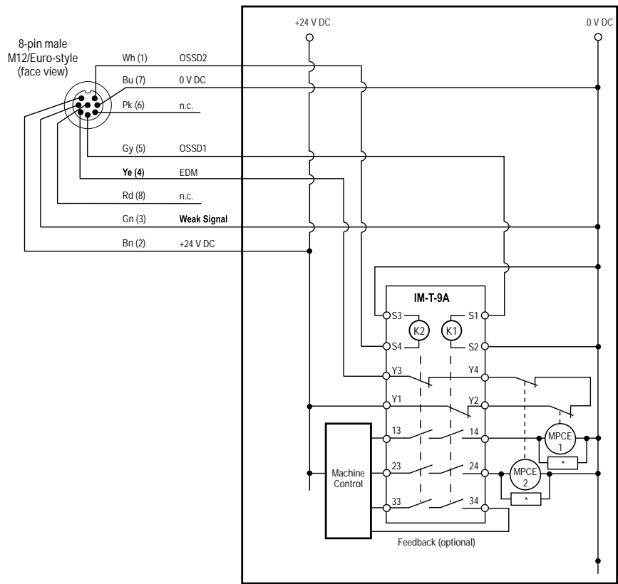
Figure 33. Generic Wiring Diagram—IM-T-9A Interface Module (1-Channel EDM)
