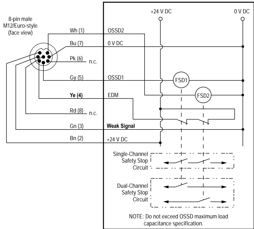
Figure 32. Generic Wiring Diagram—8-pin Receiver and Redundant FSDs
