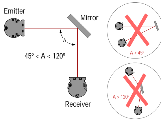
Figure 9. Using S4B sensors in a retroreflective mode
