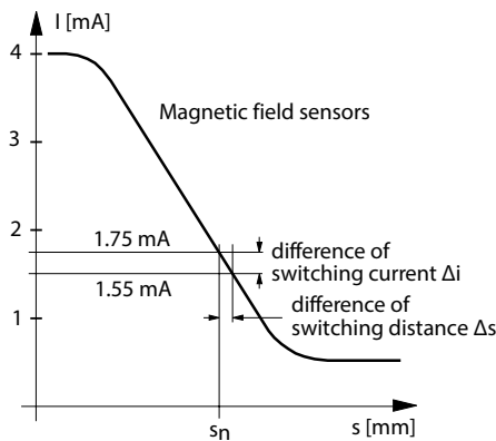
Abb. 1: NAMUR characteristic curve of the magnetic field sensors in compliance with EN 60947-5-6
