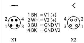
M8 × 1 Power Supply
