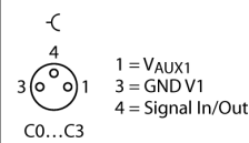
M8 × 1 I/O port
