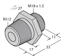
FCA-FCST-N1/2-A4 6870293
