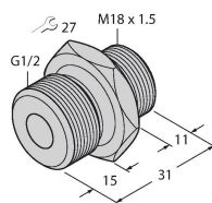
FCA-FCST-N1/2-A4 6870293
