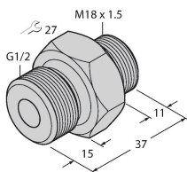
FCA-FCST-G1/2-A4/L037 6870292
