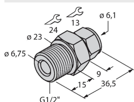
CF-M-6-G1/2-A4
