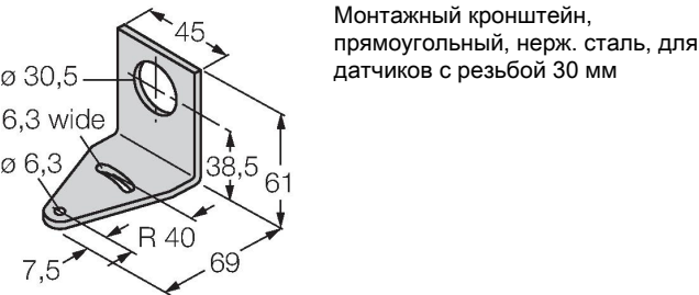
SMB30SC 3052521
