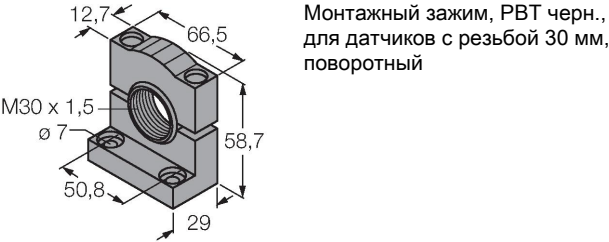
SMB30SC 3052521
