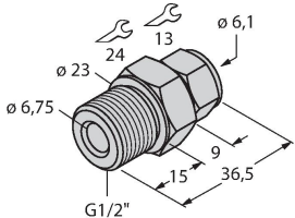
CF-M-6-G1/2-A4 9910530
