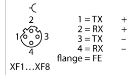
Ethernet, M12 × 1
